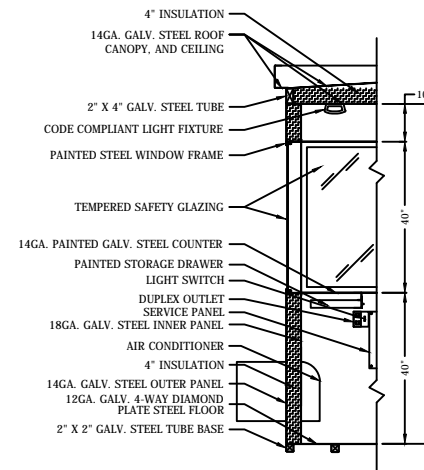
S11 SECTION NO SCALE
