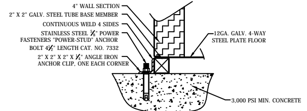
FIELD DRILLED ANCHOR BOLT DETAIL NO SCALE
